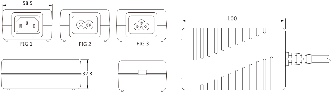
FIG 1: IEC-320-C14
