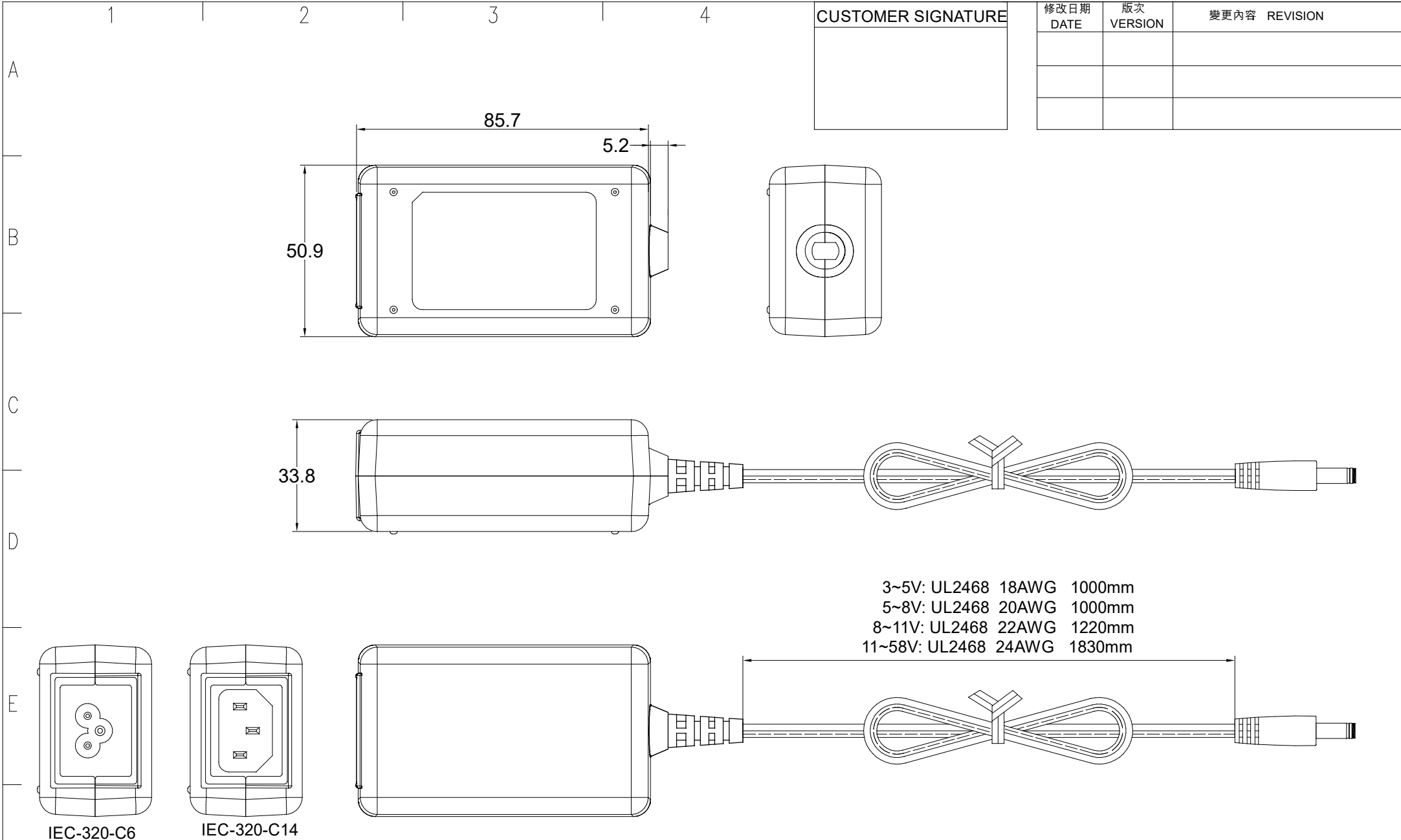
IEC-320-C6
